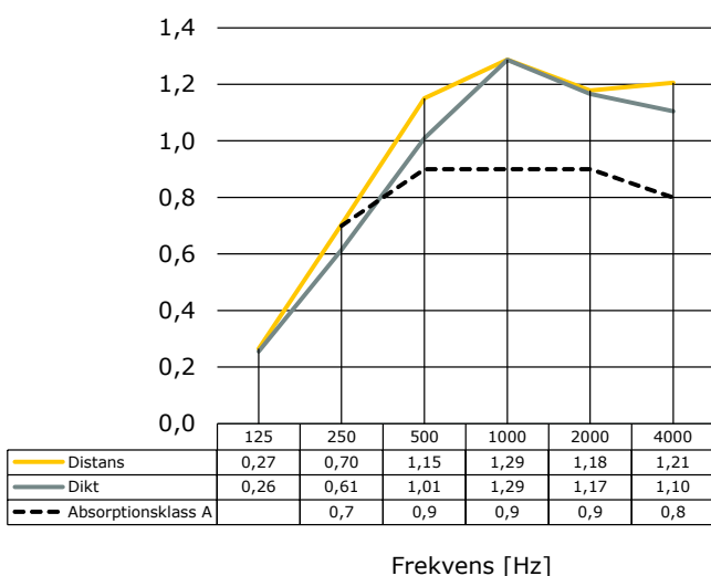
Ljudabsorptionskoefficient
